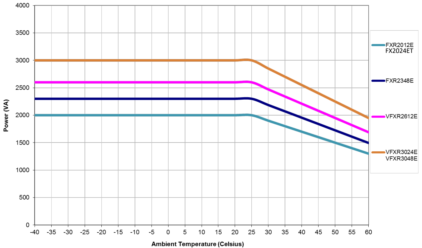
Figure 2: Power/Temperature de-rating for FXR 50Hz models
