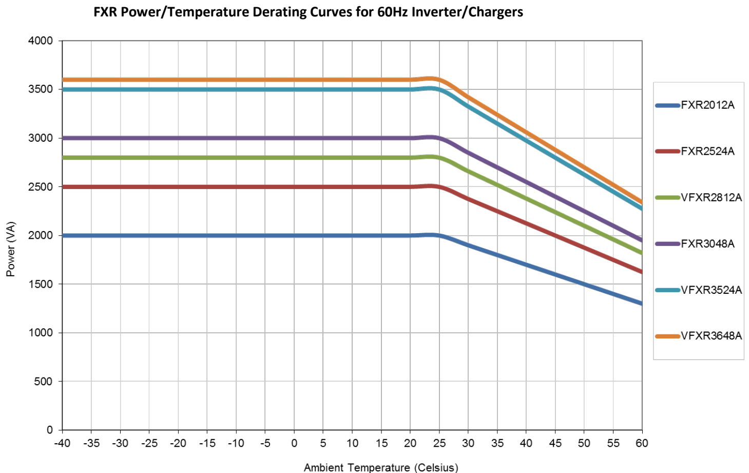
Figure 1: Power/Temperature de-rating for FXR 60Hz models
