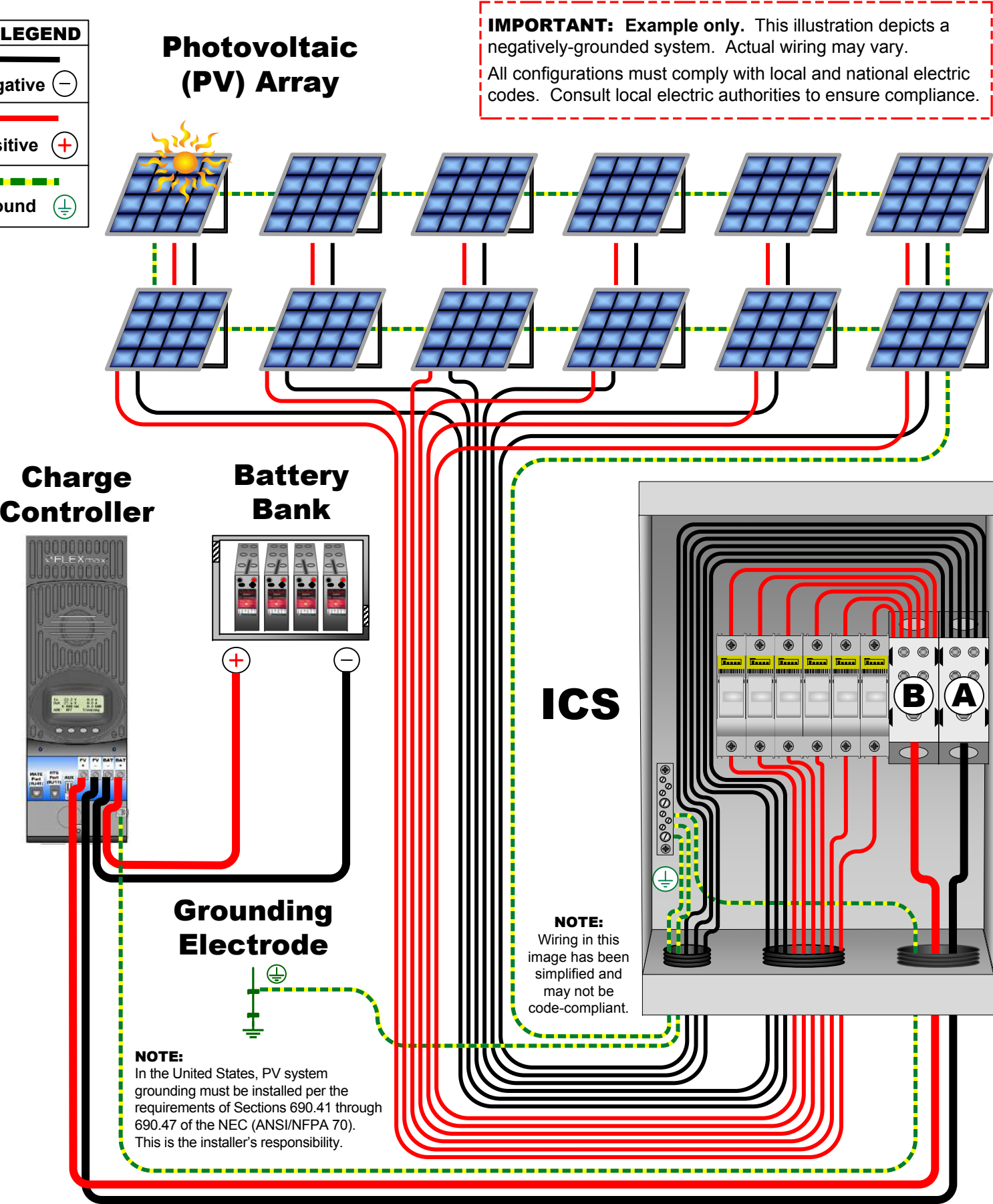
Figure 4 Wiring FW-ICS
