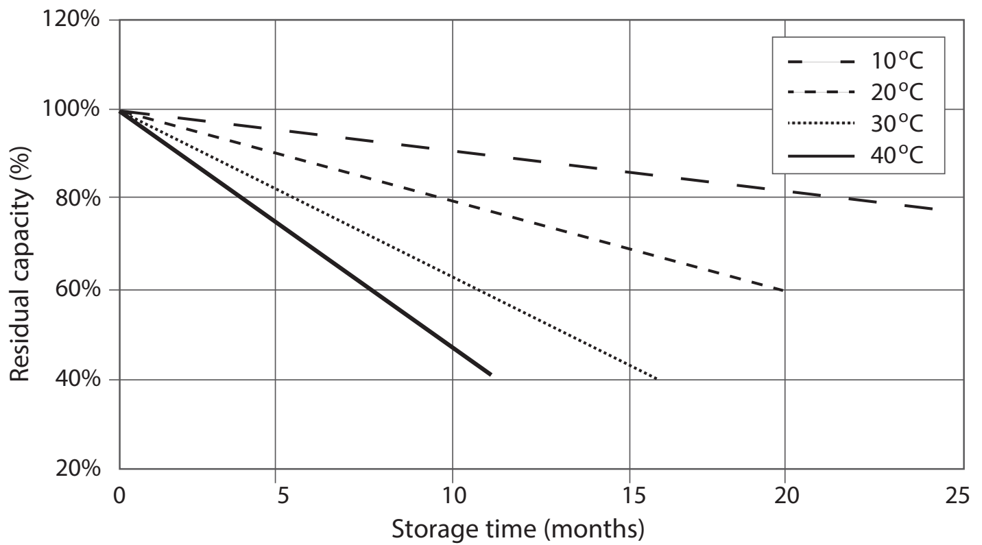
Figure 3, Self-Discharge Characteristics
