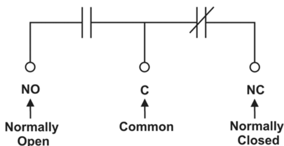
Figure 7—Showing relay connections
