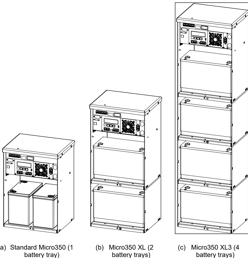
Figure 1 — Micro350 cabinets
