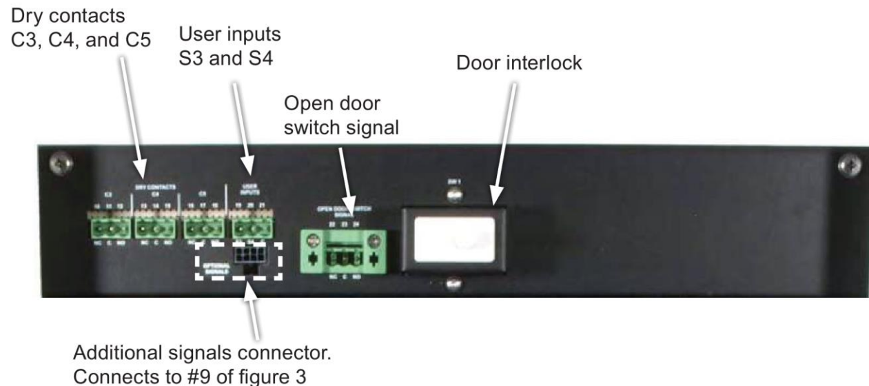
Figure 6 — Micro350 Top Panel
