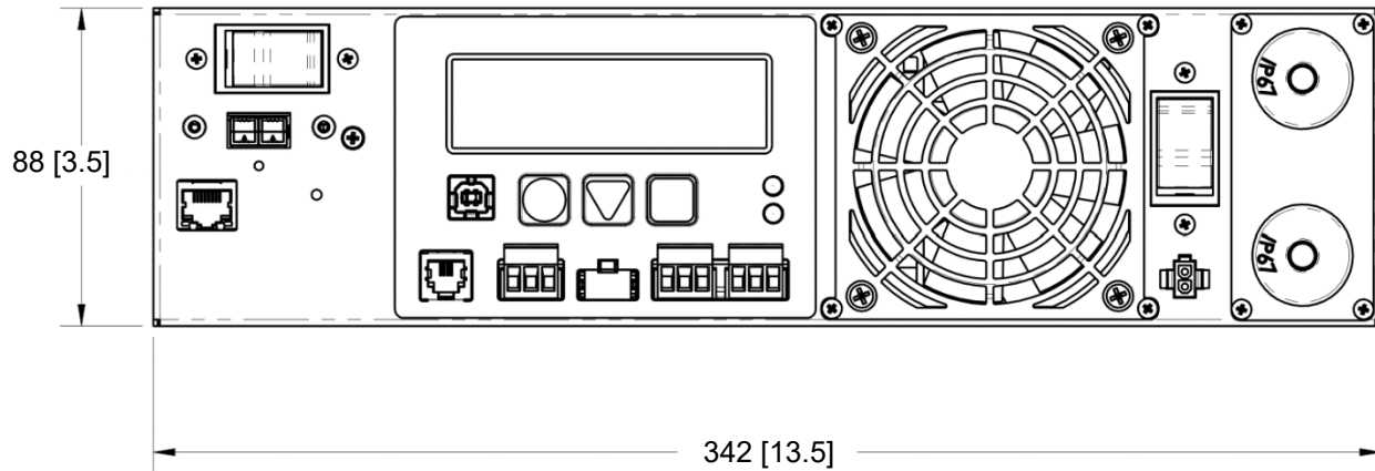
Figure 9 — FXM350 Mounting Dimensions
