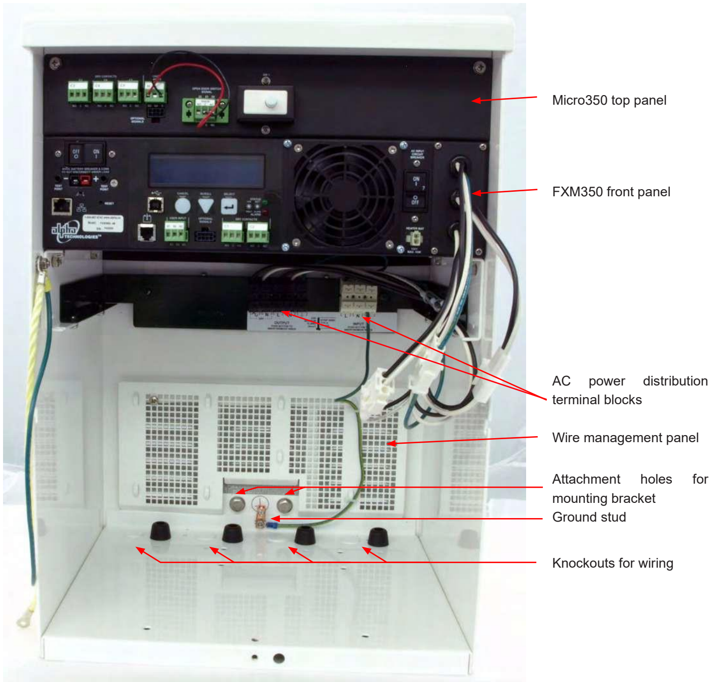
Figure 2 — FXM350 mounted in a standard Micro350 cabinet
