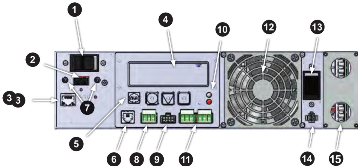
Figure 3 — FXM 350 front panel description
