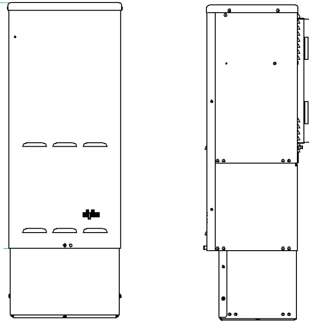
Figure 8 — Mounting on optional pedestal
