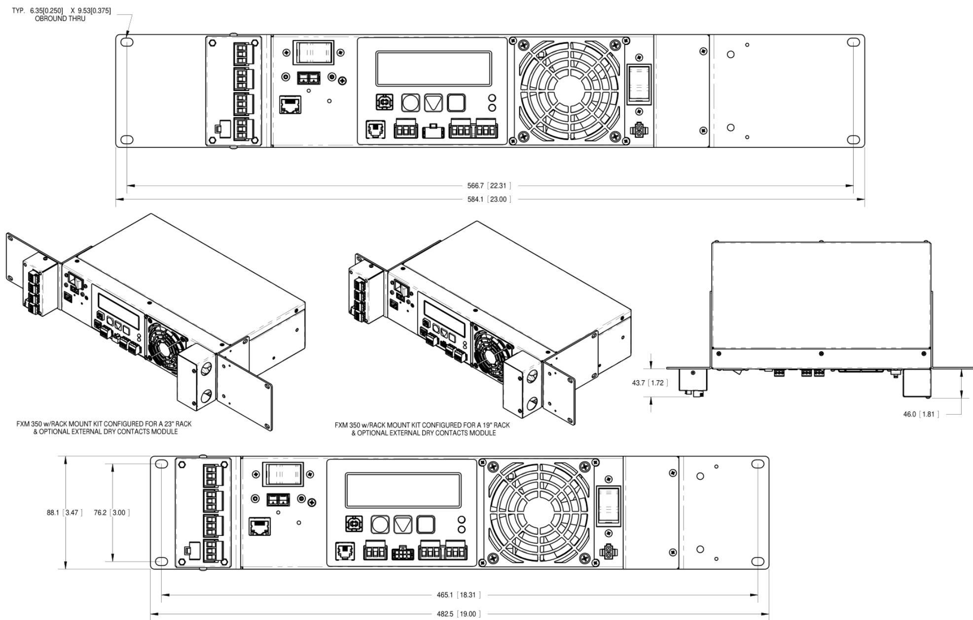
Figure 11 — FXM350 with ears for rack mounting
