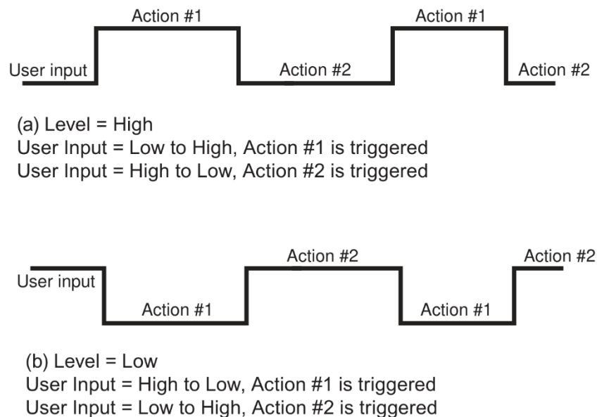
Figure 73 — Level Trigger
