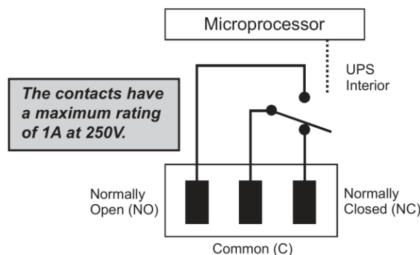
Figure 5 — Contact Layout (Standard for C1 and C2)
